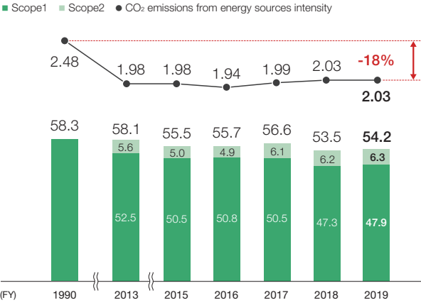
CO 2 emissions from energy sources (million t-CO 2 ) and CO 2 emission intensity (t-CO 2 /t-s) of JFE Steel
