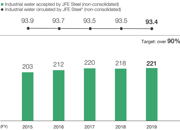
Industrial water accepted (million tons) and circulated (%) of JFE Steel
